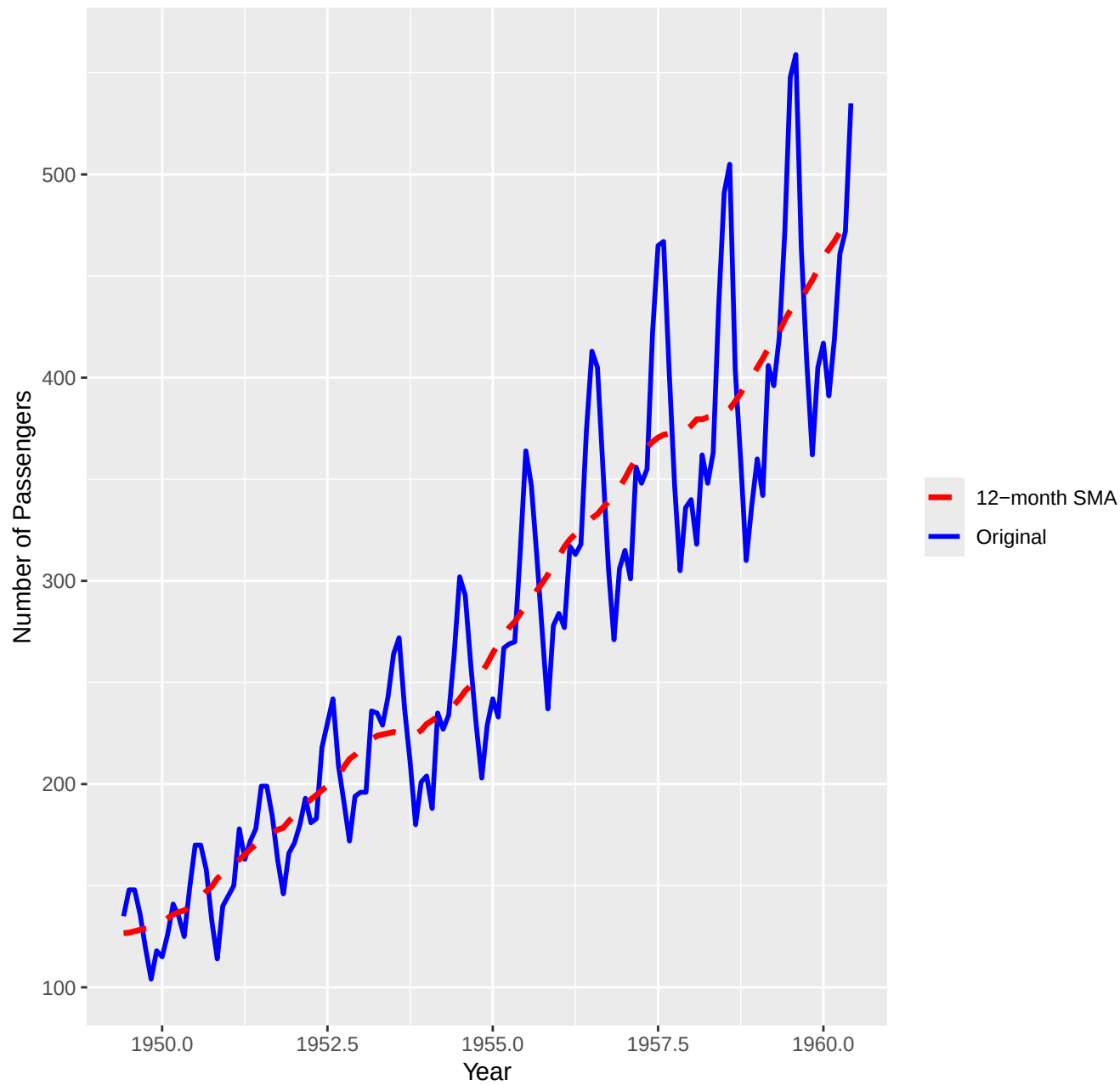
AirPassengers Data with 12-Month SMA
